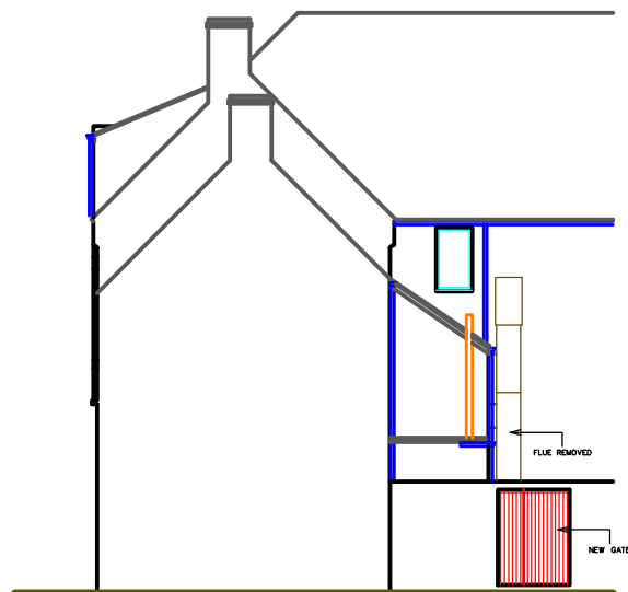
PROPOSED REAR (NORTH WEST) ELEVATION
